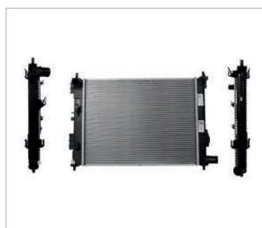
RADIADOR AGUA C/S AIRE STD 520*400*16MM (ACCENT 1.6L 18-22) SE-DAN/H-BACK T/S/O
