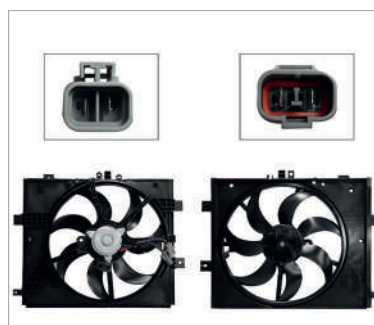
MOTOVENTI COMPLETO C/S AIRE C/T 2PIN S/RES 2CONECTORES 7ASPAS V-DRIVE/MARCH/NOTE
